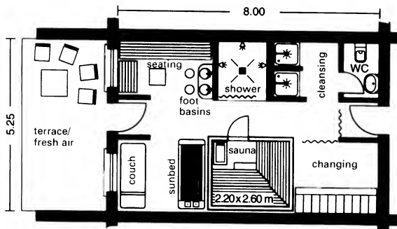
⑦ Hotel sauna 5.25 x 8.00 m
